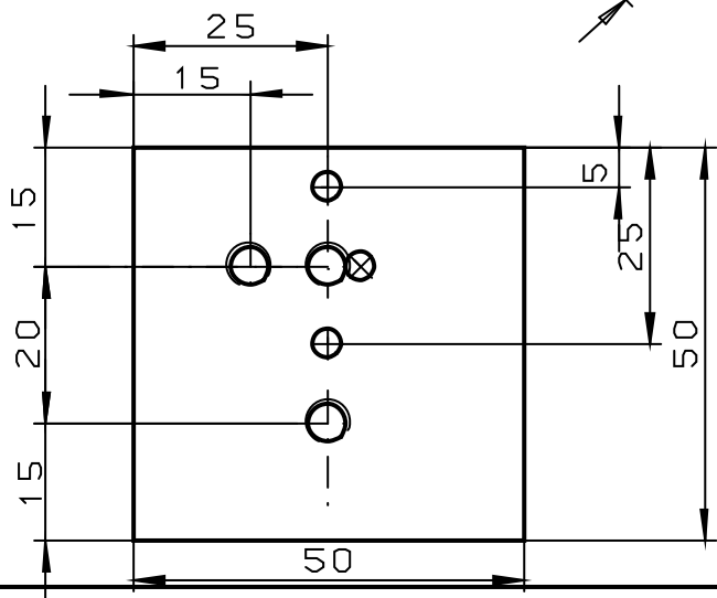
Adapterplatte t=10
